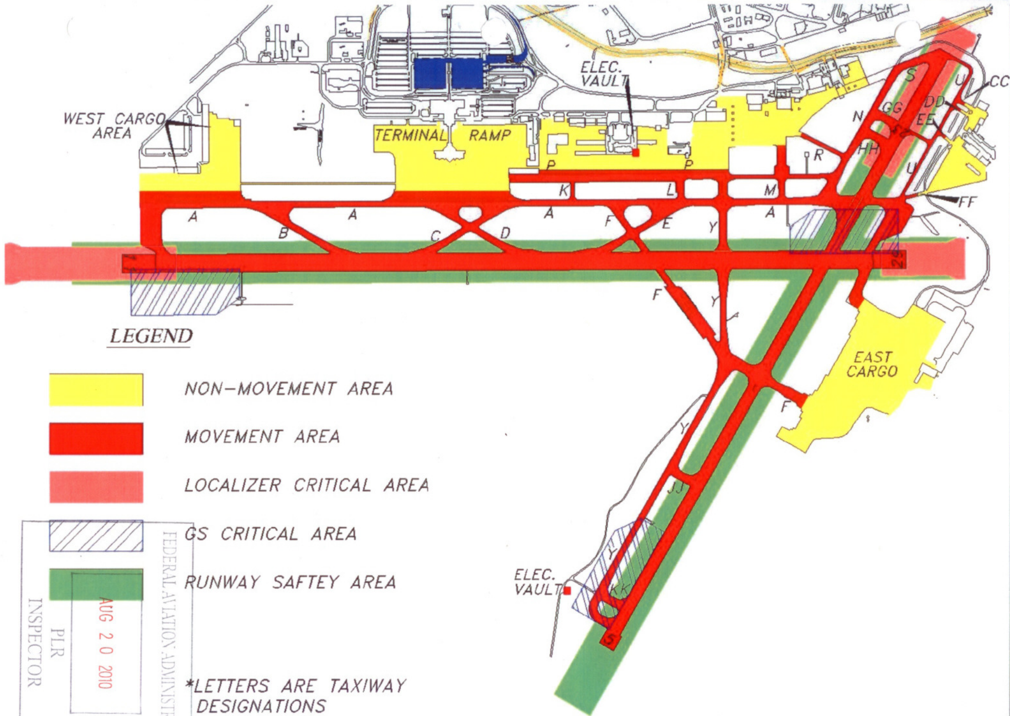
EXHIBIT 5, RUNWAY, TAXIWAY AND MOVEMENT/NONMOVEMENT AREA CHART
